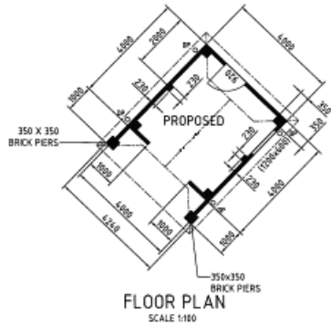
Typical Layout for an Outbuilding
